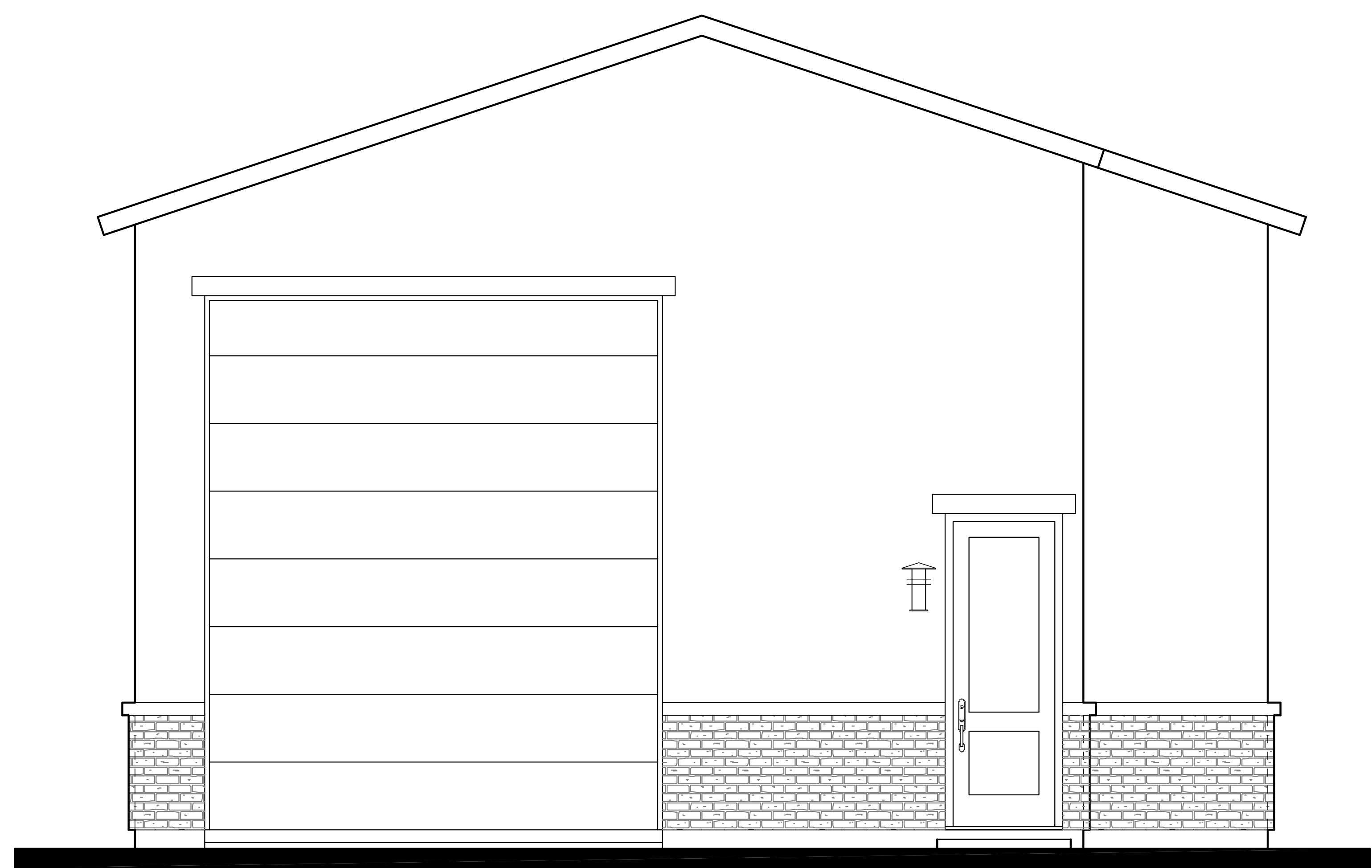
NORTH ELEVATION
