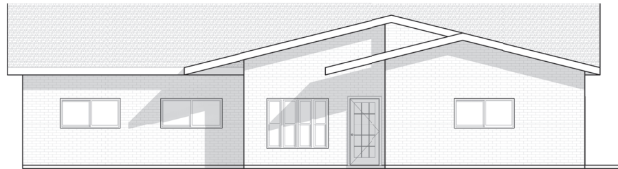
② FRONT VIEW 1/4" = 1'-0"
