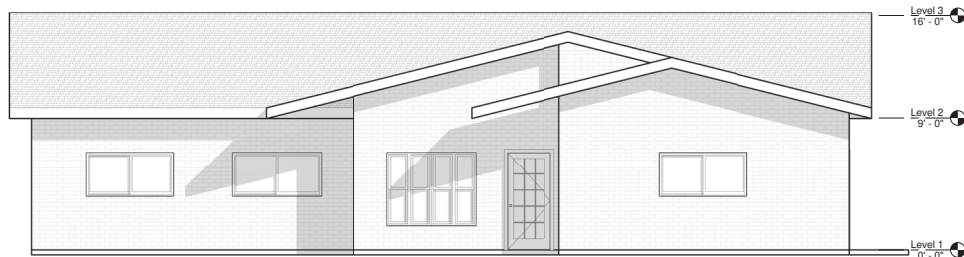
③ PROP. FRONT ELEVATION 1/4" = 1'-0"
