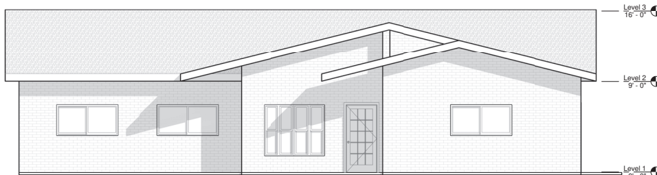
① PROP. SOUTH ELEVATION 1/4" = 1'-0"
