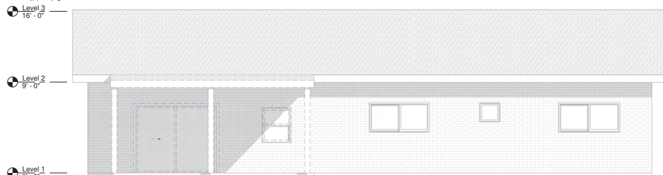
② EXIS - DEMO REAR ELEVATION 1/4" = 1'-0"
