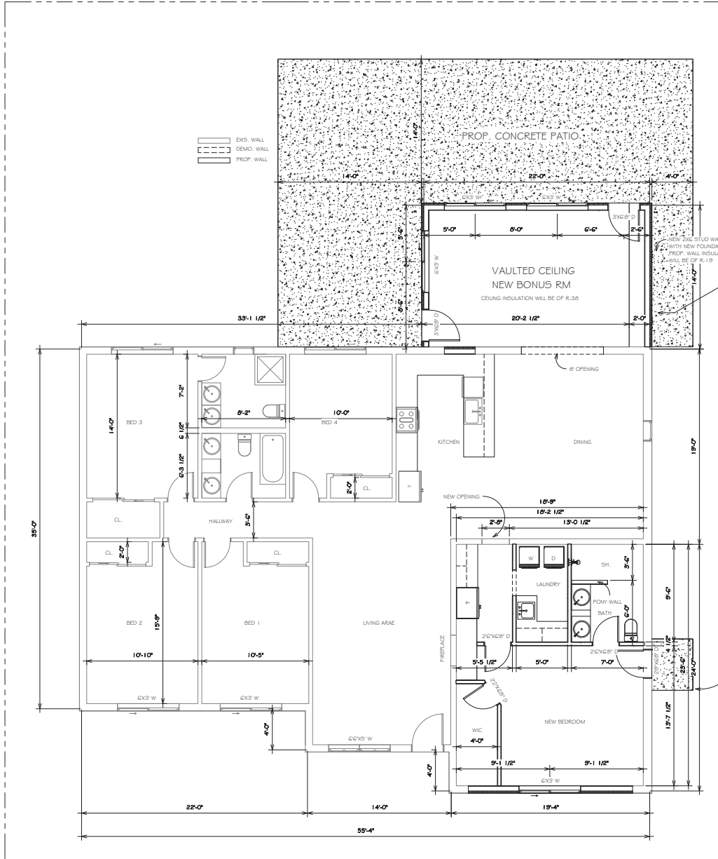
① PROP. PLAN 1/4" = 1'-0"
