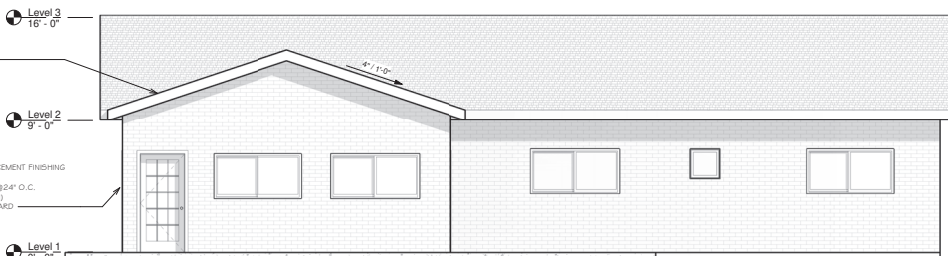
② PROP. NORTH ELEVATION 1/4" = 1'-0"
