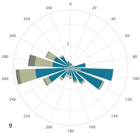
Figure 9: Wind directions.
