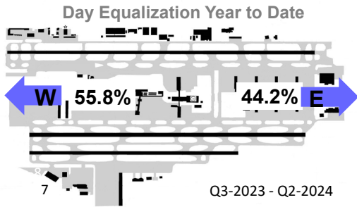
Figure 7: Day equalization.
