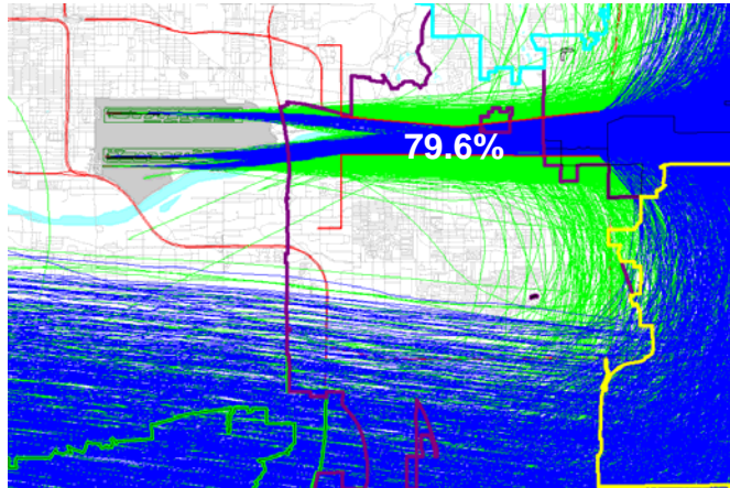
Corridor Compliance: The depiction includes some erroneous diagonal track patterns.
