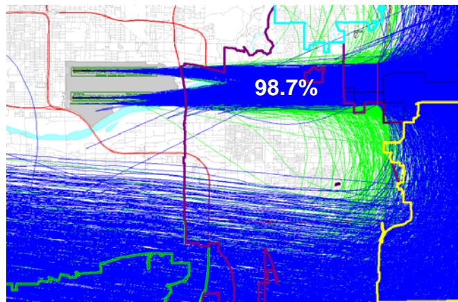
Gate Compliance – The depiction includes some erroneous diagonal track patterns.
