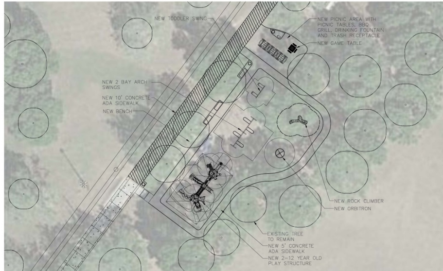
SVOB PARK LAYOUT PLAN 'A'
