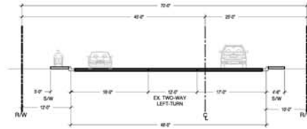
SEGMENT PURPLE EXISTING (70' -0" R/W)
