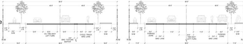
SEGMENT TYPE 06-1 ALTERNATIVE - 1 (PURPLE) CYCLE TRACK OPT.
