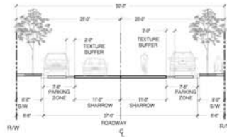
SEGMENT TYPE 04-3 ALTERNATIVE - 3 50' -0" R/W - PARKING (YELLOW)
