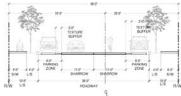
SEGMENT TYPE 04-1 ALTERNATIVE - 1 58' -0" R/W - PARKING (YELLOW)
