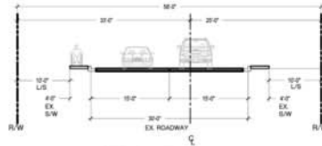
SEGMENT YELLOW EXISTING 58' -0" R/W
