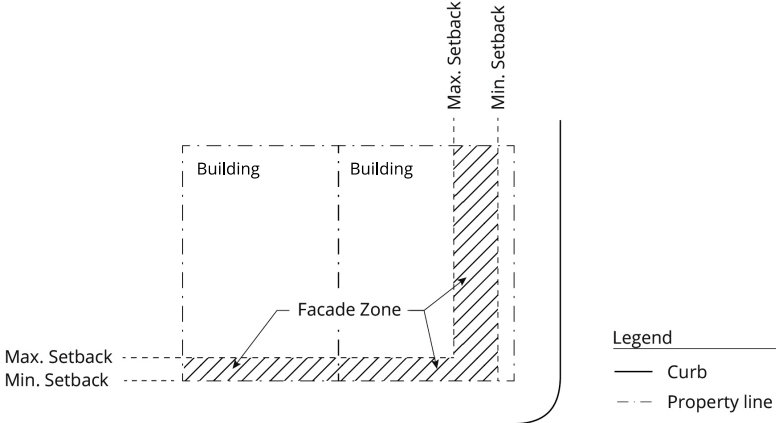
Figure 7-107A. Façade Zone
