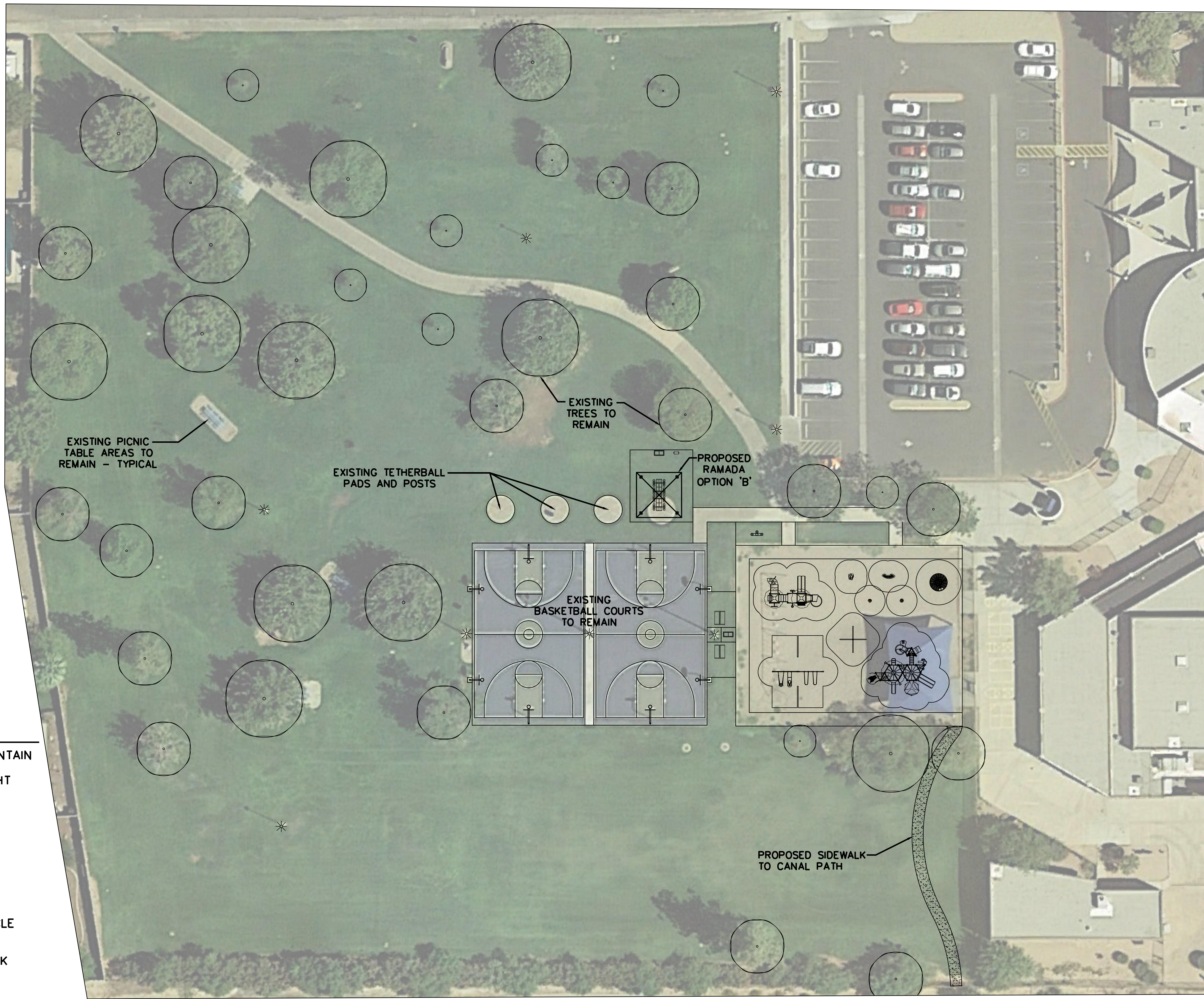
REDDEN PARK PLAYGROUND LAYOUT OPTION A
