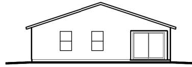
SOUTH ELEVATION ELEVATION C 1/8" = 1'-0"
