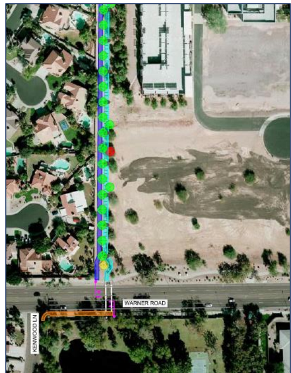
Proposed 30% Design showing pedestrian signal alignment just east of Kenwood Lane, directly connecting to the multi-use path and equestrian trail on the West side of ASU Research Park
