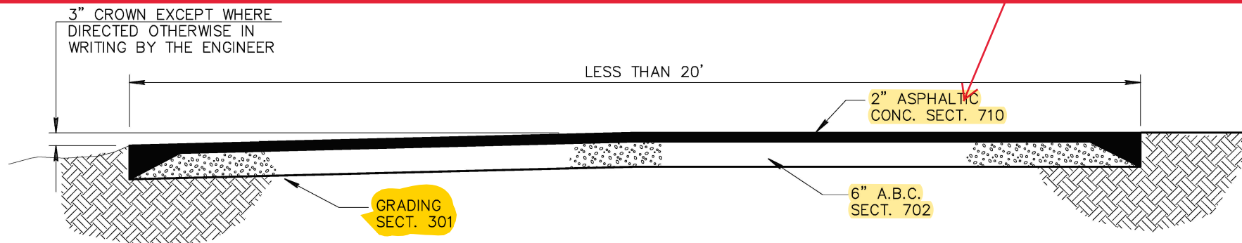
RESIDENTIAL ALLEY DETAIL
