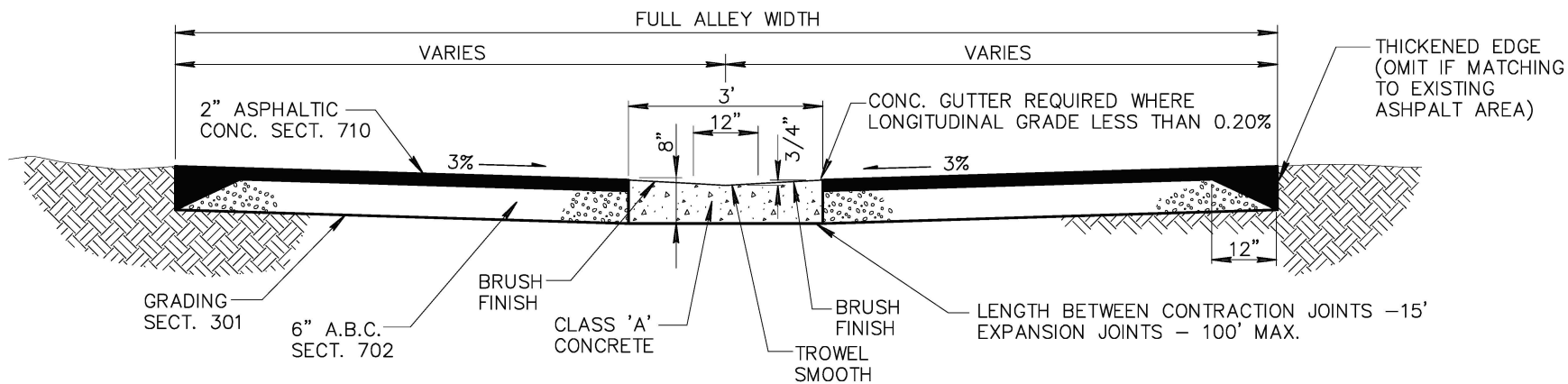
PAVED ALLEY DETAIL
