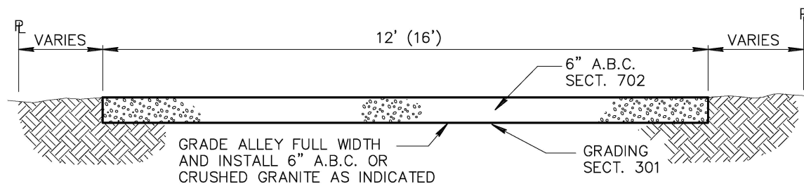
UNPAVED ALLEY DETAIL
